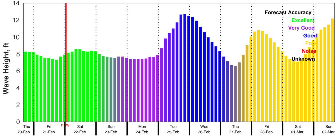
CMEMS Wave Forecast for NDBC 46028 from 20-Feb-2025 16:00:00 to 02-Mar-2025 16:00:00
