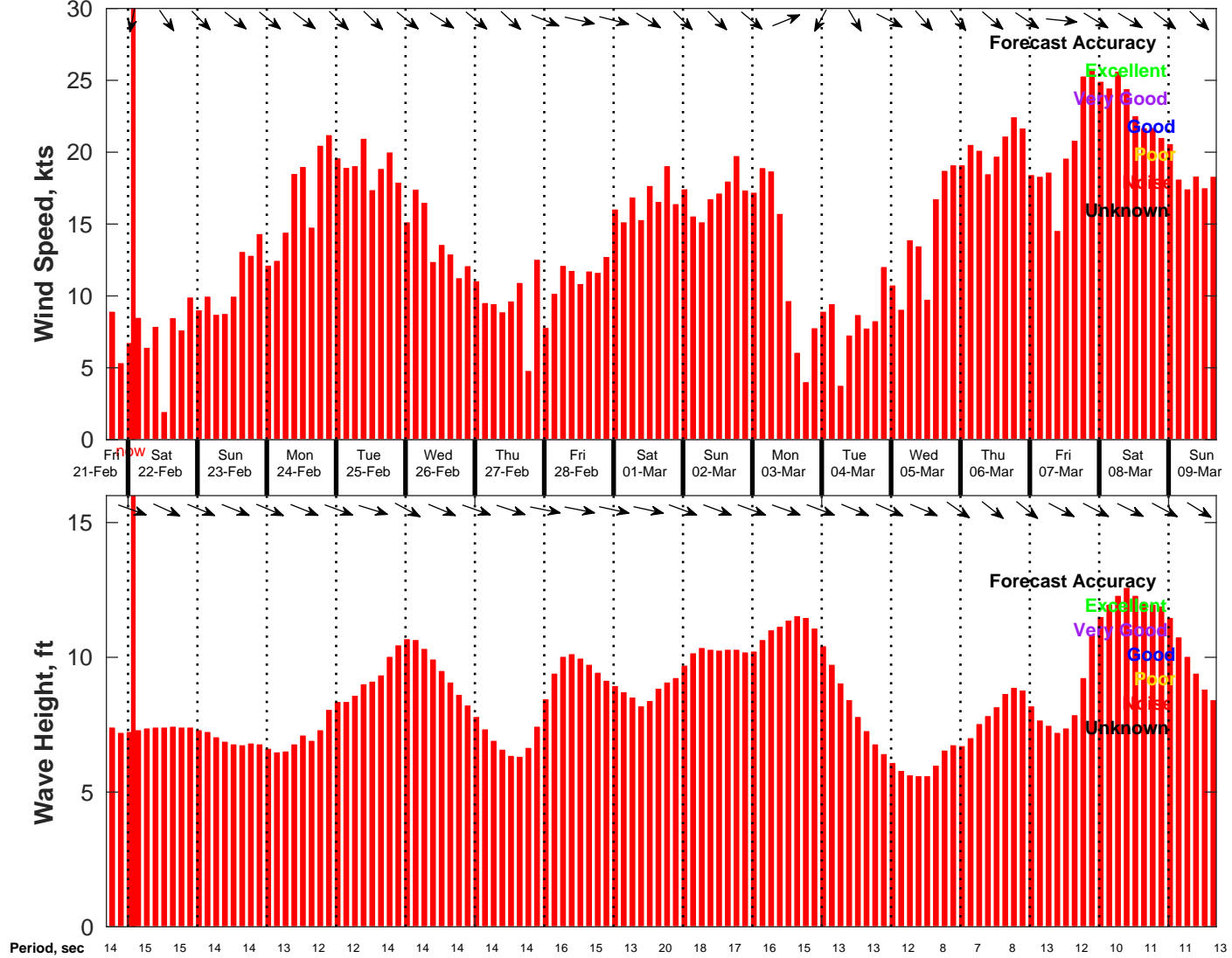
Wind & Wave Forecast for NDBC 46053 from 21-Feb-2025 17:00:00 to 09-Mar-2025 17:00:00
