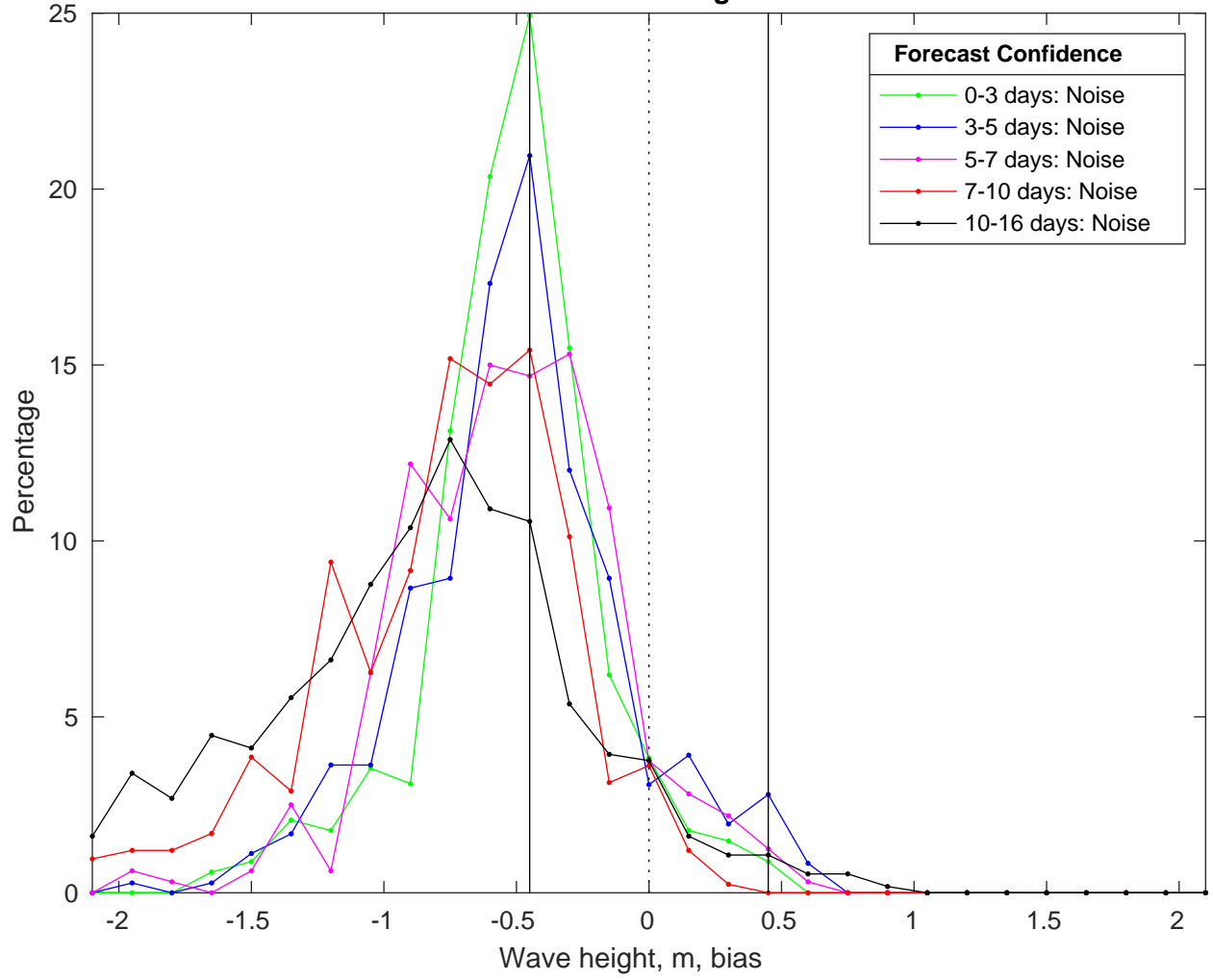
NDBC 46054 vs GFS Waves Bias Histogram: 22-Feb-2025
