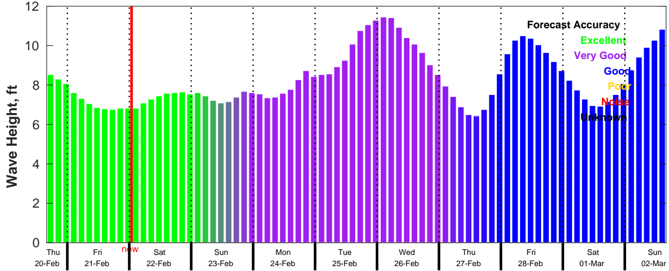
CMEMS Wave Forecast for NDBC 46054 from 20-Feb-2025 16:00:00 to 02-Mar-2025 16:00:00
