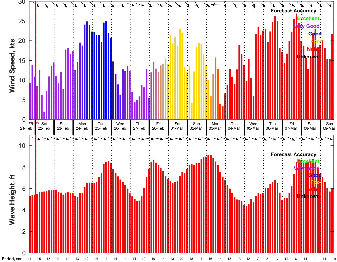
Wind & Wave Forecast for NDBC 46054 from 21-Feb-2025 16:00:00 to 09-Mar-2025 16:00:00
