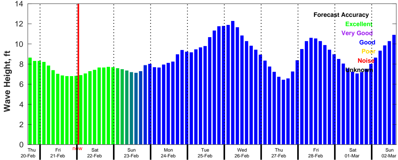
CMEMS Wave Forecast for NDBC 46069 from 20-Feb-2025 16:00:00 to 02-Mar-2025 16:00:00
