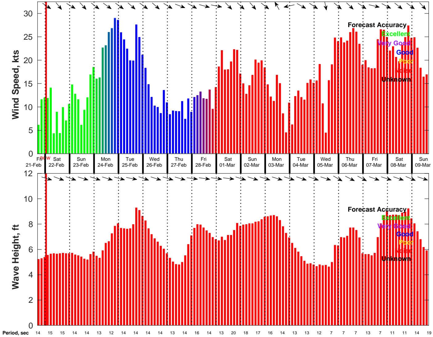
Wind & Wave Forecast for NDBC 46069 from 21-Feb-2025 16:00:00 to 09-Mar-2025 16:00:00
