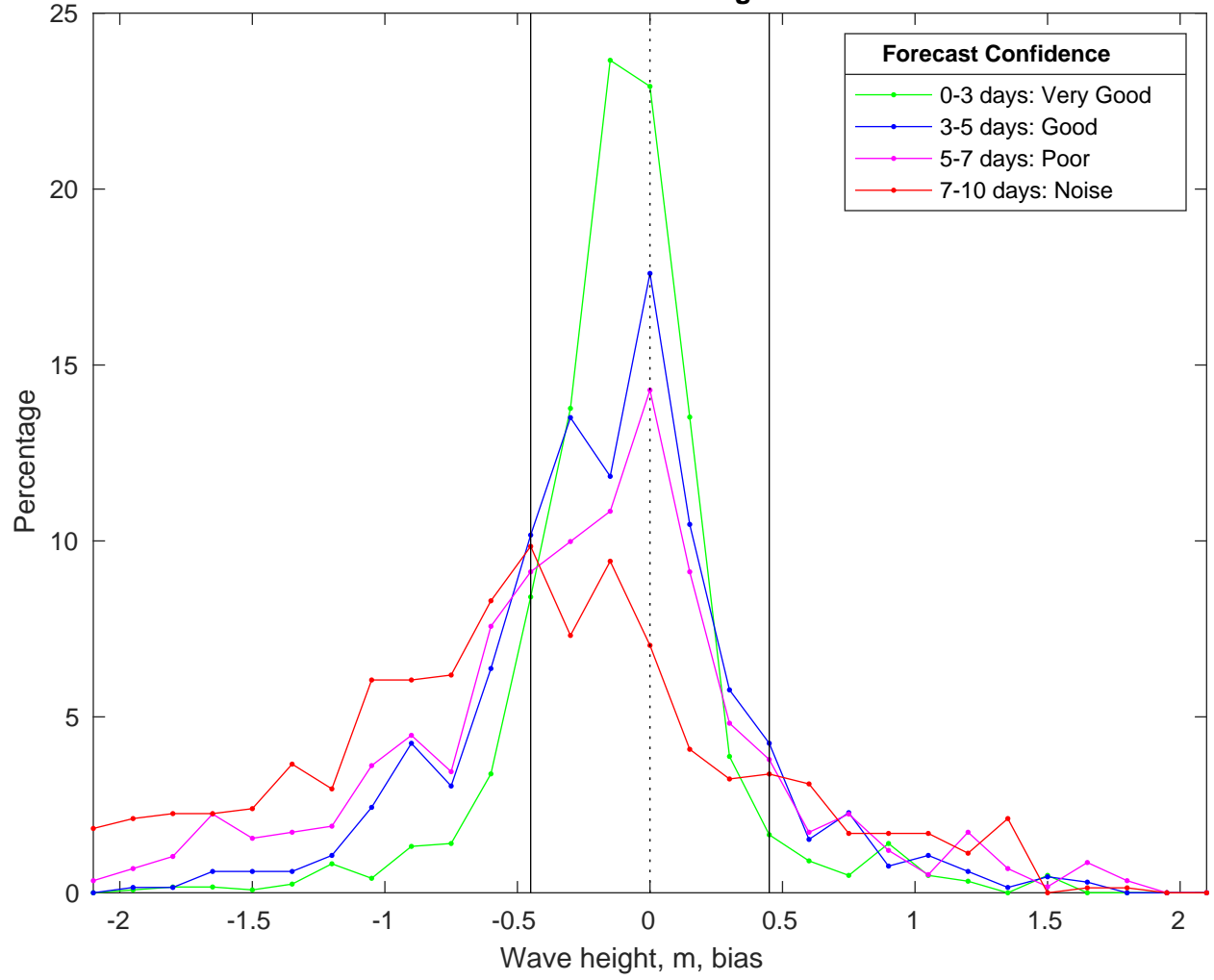
NDBC 46246 vs CMEMS Waves Bias Histogram: 22-Feb-2025
