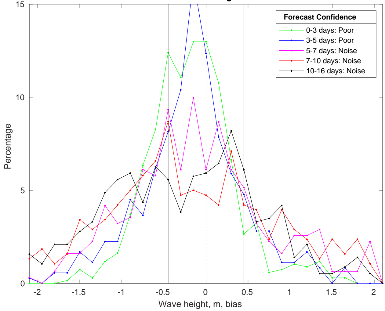
NDBC 46246 vs GFS Waves Bias Histogram: 22-Feb-2025
