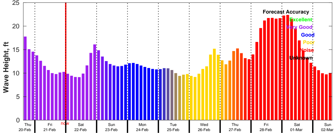
CMEMS Wave Forecast for NDBC 46246 from 20-Feb-2025 15:00:00 to 02-Mar-2025 15:00:00
