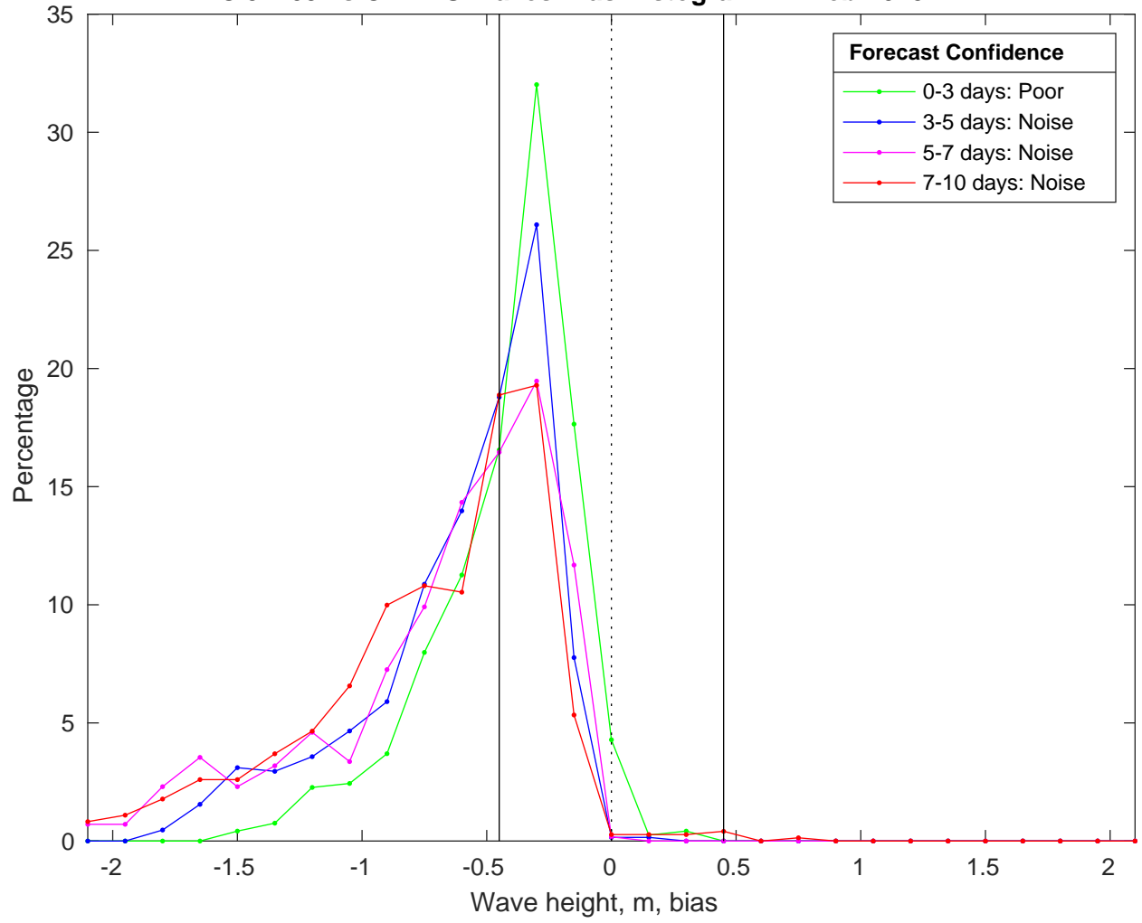
NDBC 51209 vs CMEMS Waves Bias Histogram: 22-Feb-2025
