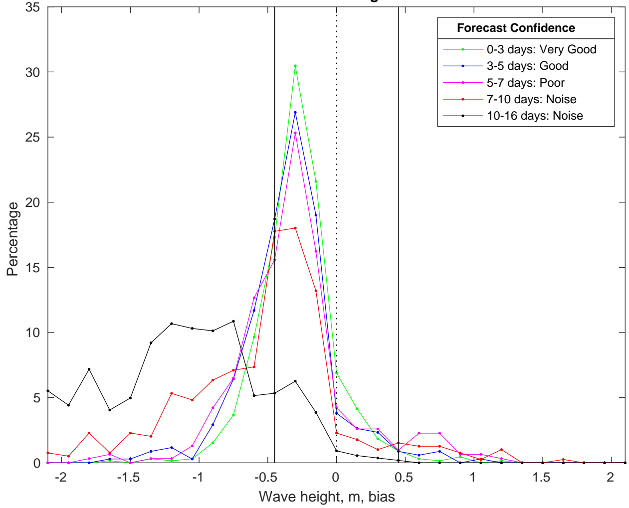
NDBC 51209 vs GFS Waves Bias Histogram: 22-Feb-2025
