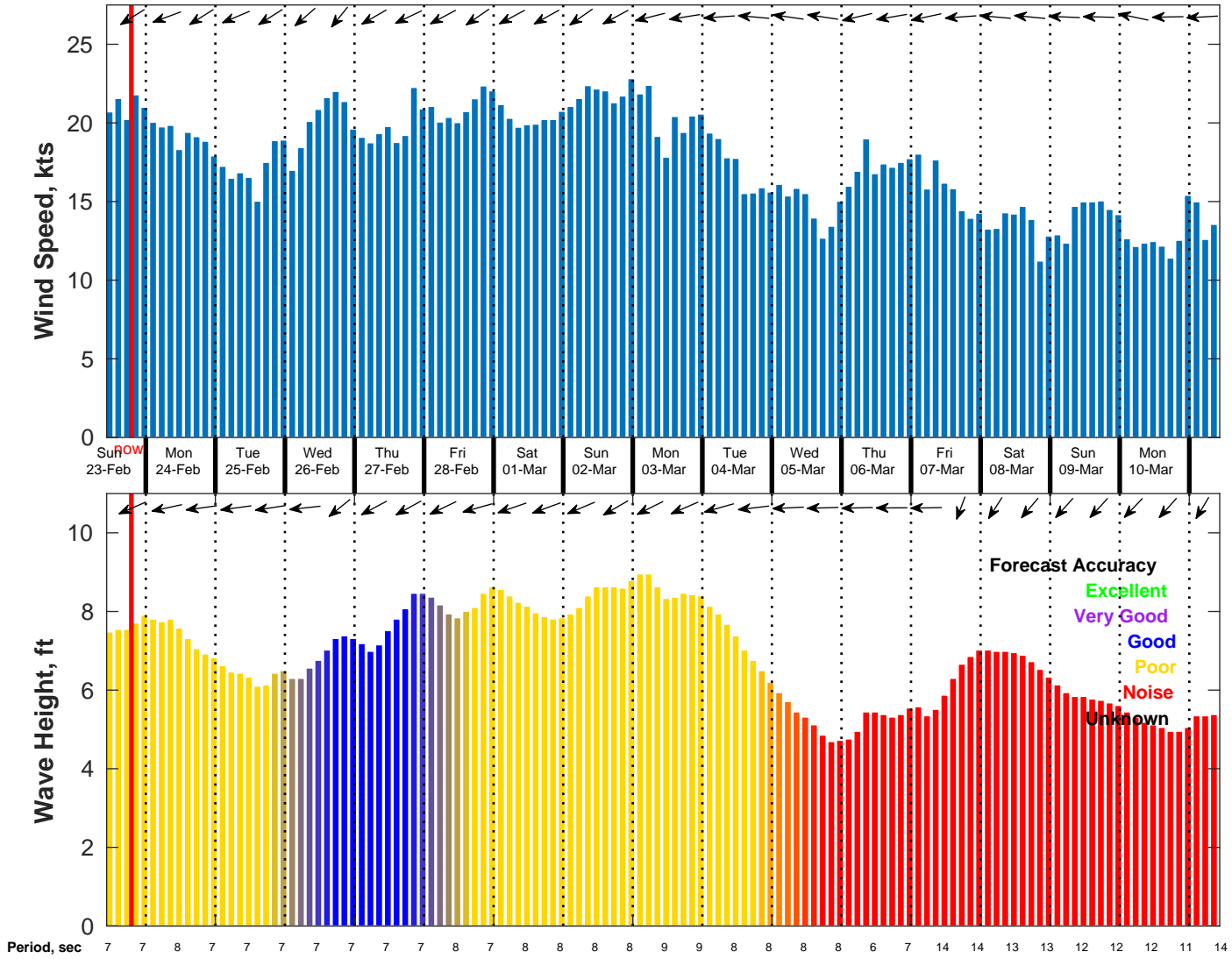
Wind & Wave Forecast for NDBC 52211 from 22-Feb-2025 10:00:00 to 10-Mar-2025 10:00:00
