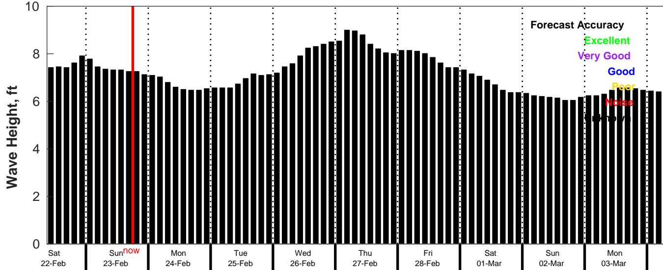
CMEMS Wave Forecast for NDBC 52212 from 21-Feb-2025 09:00:00 to 03-Mar-2025 09:00:00
