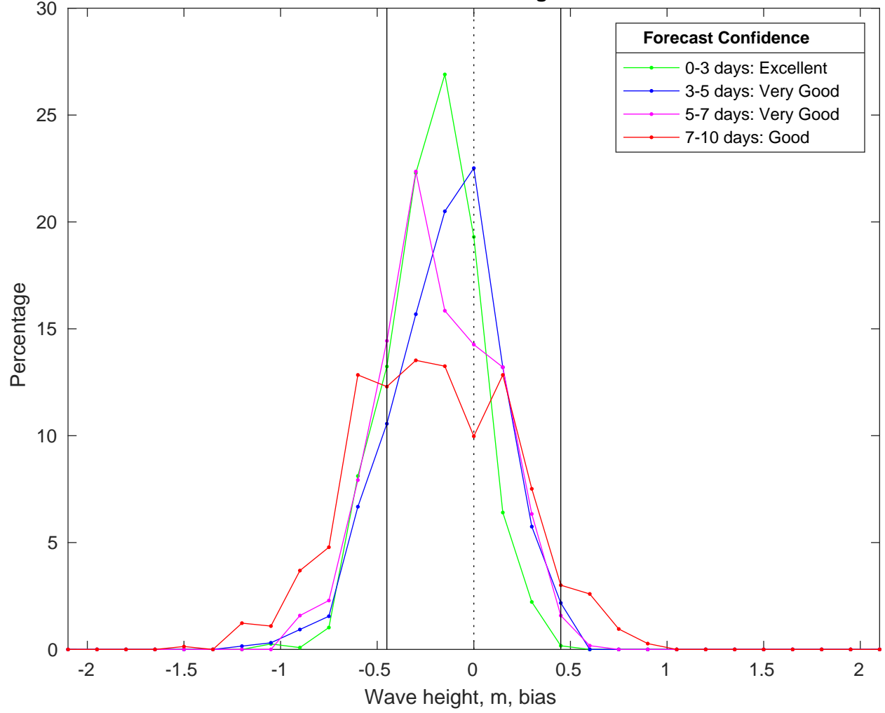
NDBC 52213 vs CMEMS Waves Bias Histogram: 22-Feb-2025
