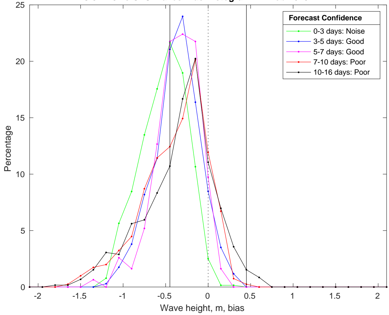
NDBC 52213 vs GFS Waves Bias Histogram: 22-Feb-2025
