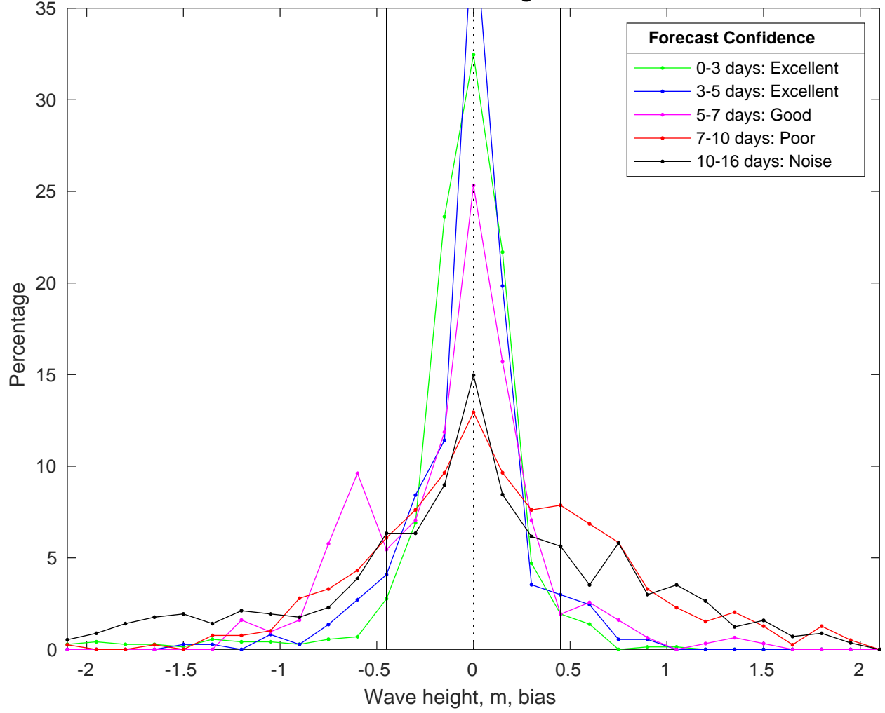
NDBC 41004 vs GFS Waves Bias Histogram: 23-Feb-2025
