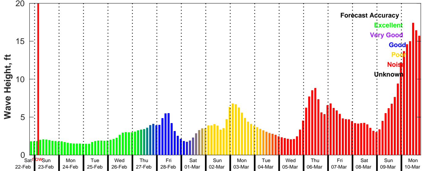
GFS Wave Forecast for NDBC 41004 from 22-Feb-2025 19:00:00 to 10-Mar-2025 19:00:00
