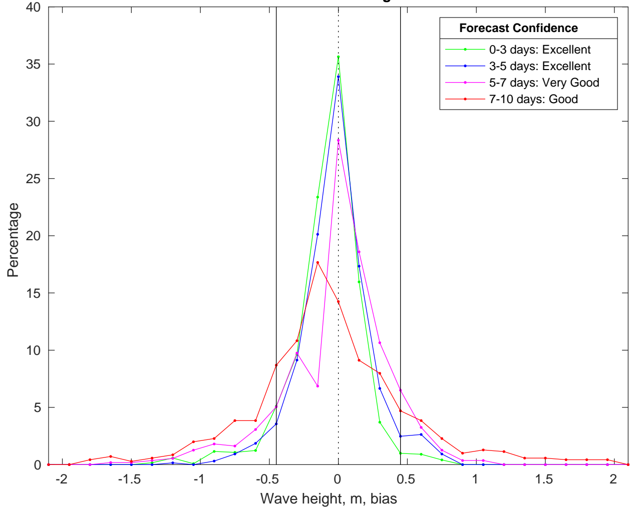
NDBC 41013 vs CMEMS Waves Bias Histogram: 23-Feb-2025
