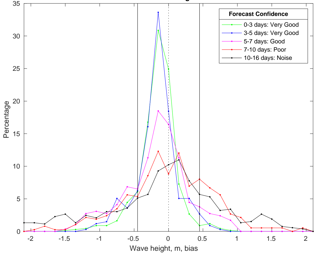
NDBC 41013 vs GFS Waves Bias Histogram: 23-Feb-2025
