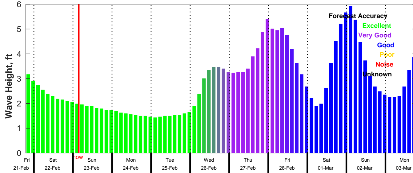
CMEMS Wave Forecast for NDBC 41013 from 21-Feb-2025 19:00:00 to 03-Mar-2025 19:00:00
