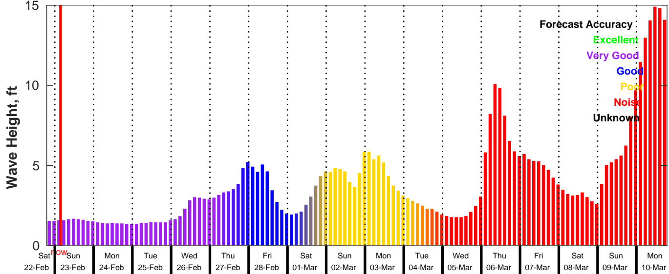
GFS Wave Forecast for NDBC 41013 from 22-Feb-2025 19:00:00 to 10-Mar-2025 19:00:00
