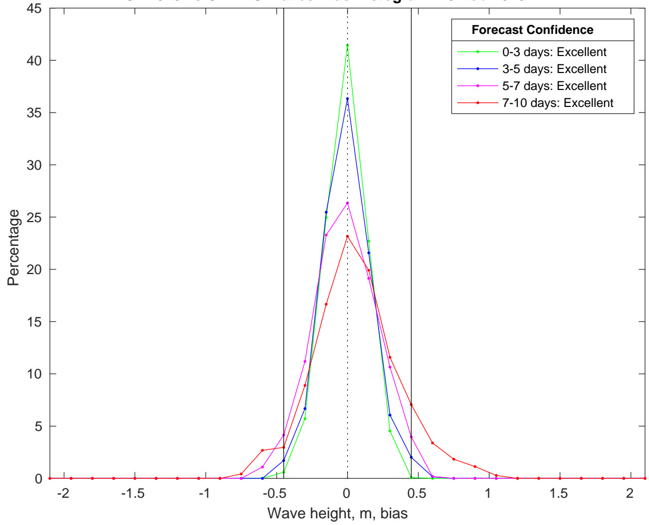
NDBC 41040 vs CMEMS Waves Bias Histogram: 23-Feb-2025
