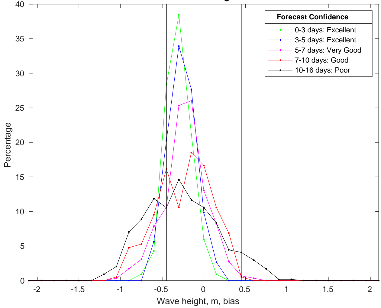
NDBC 41040 vs GFS Waves Bias Histogram: 23-Feb-2025
