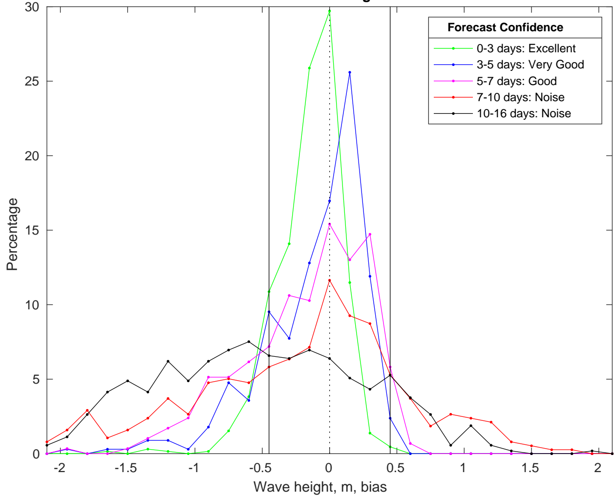
NDBC 42019 vs GFS Waves Bias Histogram: 23-Feb-2025
