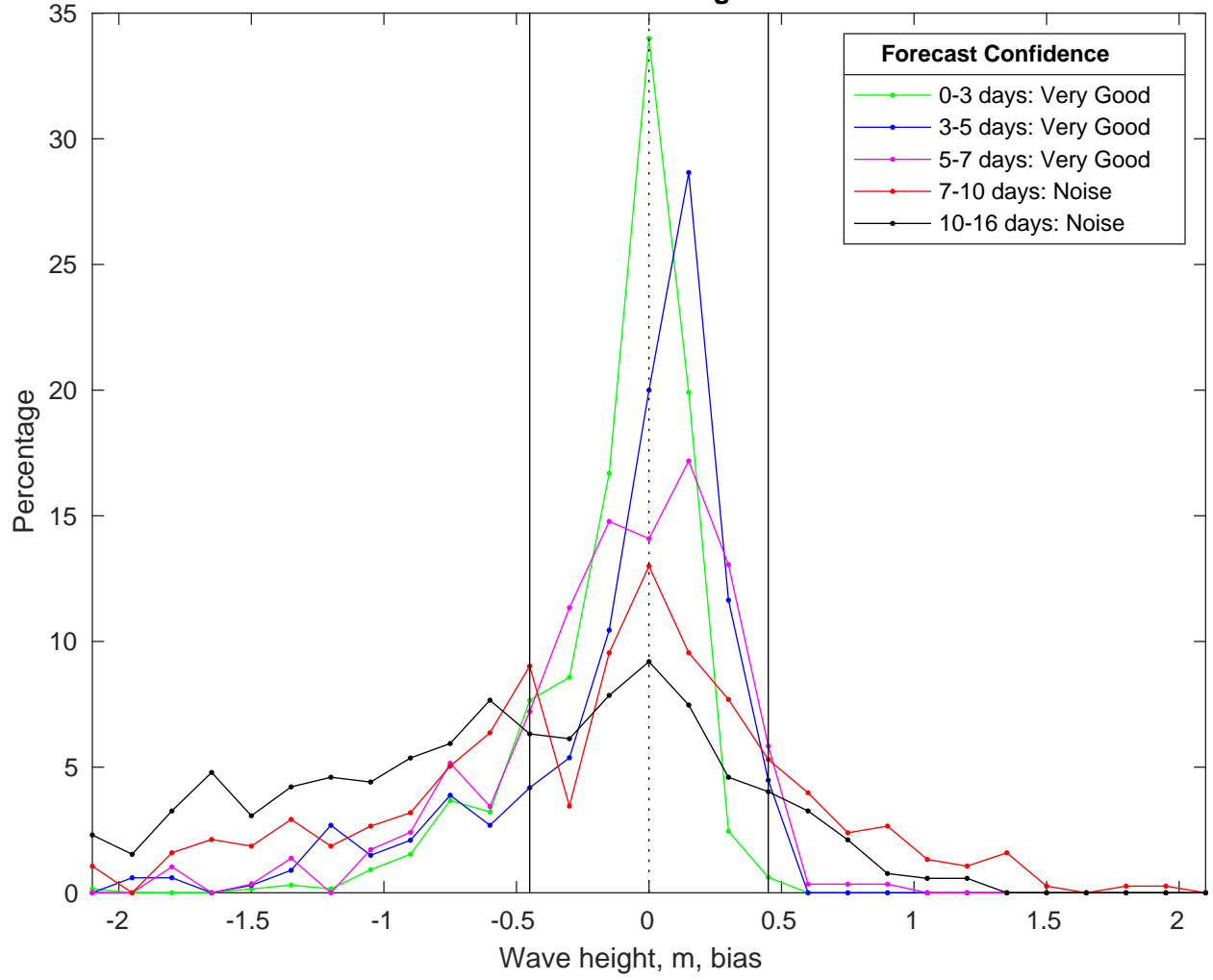
NDBC 42020 vs GFS Waves Bias Histogram: 23-Feb-2025
