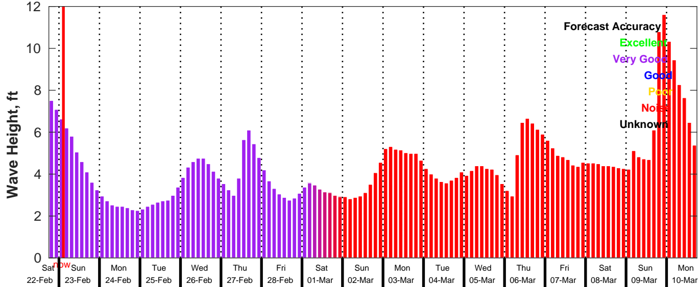
GFS Wave Forecast for NDBC 42020 from 22-Feb-2025 18:00:00 to 10-Mar-2025 18:00:00
