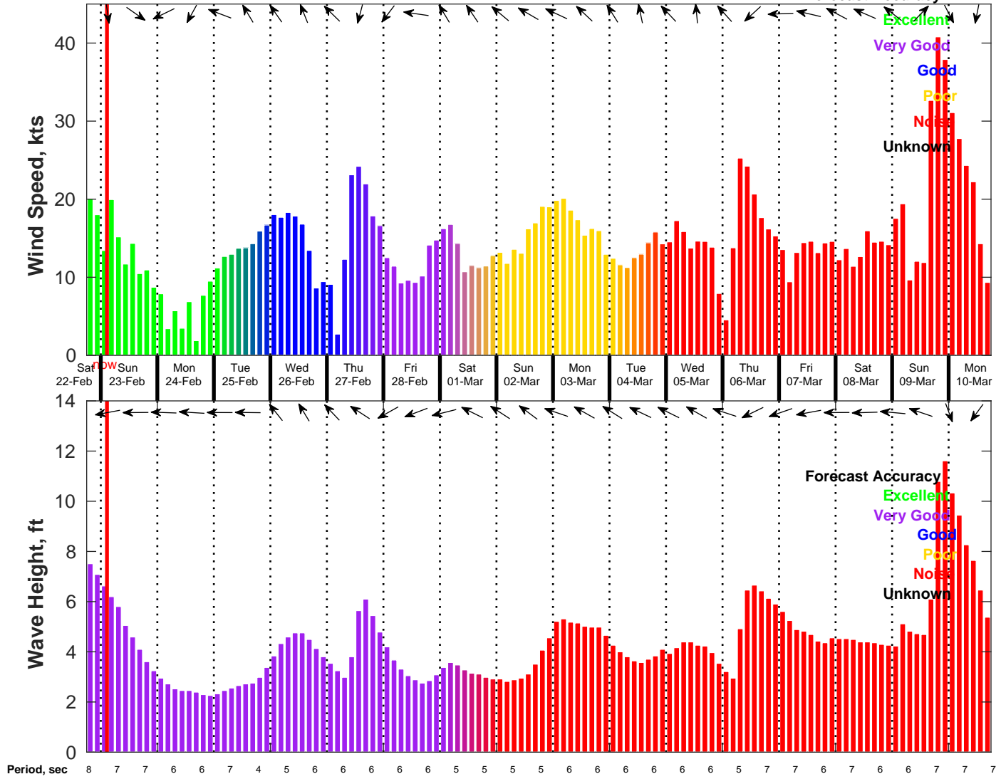
Wind & Wave Forecast for NDBC 42020 from 22-Feb-2025 18:00:00 to 10-Mar-2025 18:00:00
