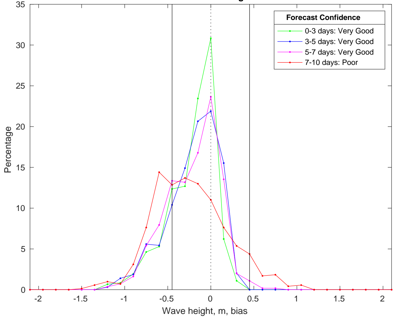
NDBC 42035 vs CMEMS Waves Bias Histogram: 23-Feb-2025
