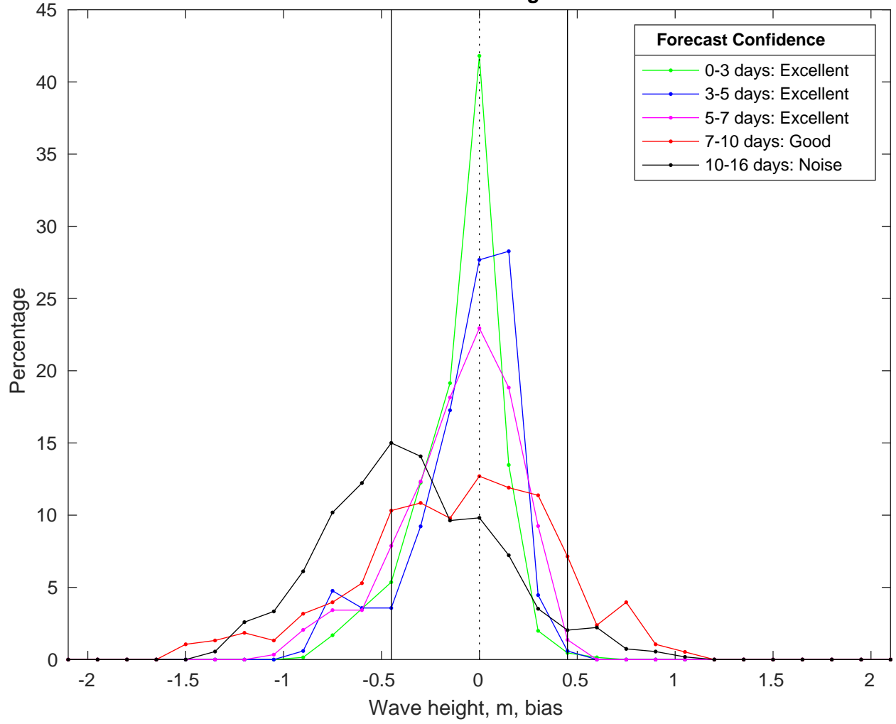
NDBC 42035 vs GFS Waves Bias Histogram: 23-Feb-2025
