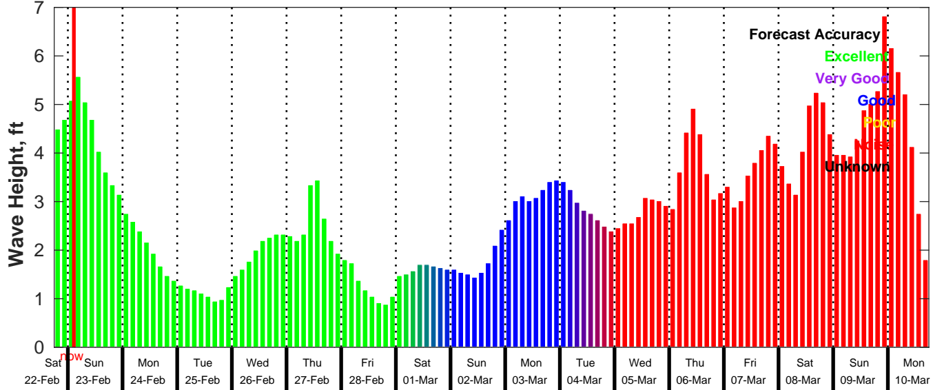
GFS Wave Forecast for NDBC 42035 from 22-Feb-2025 18:00:00 to 10-Mar-2025 18:00:00
