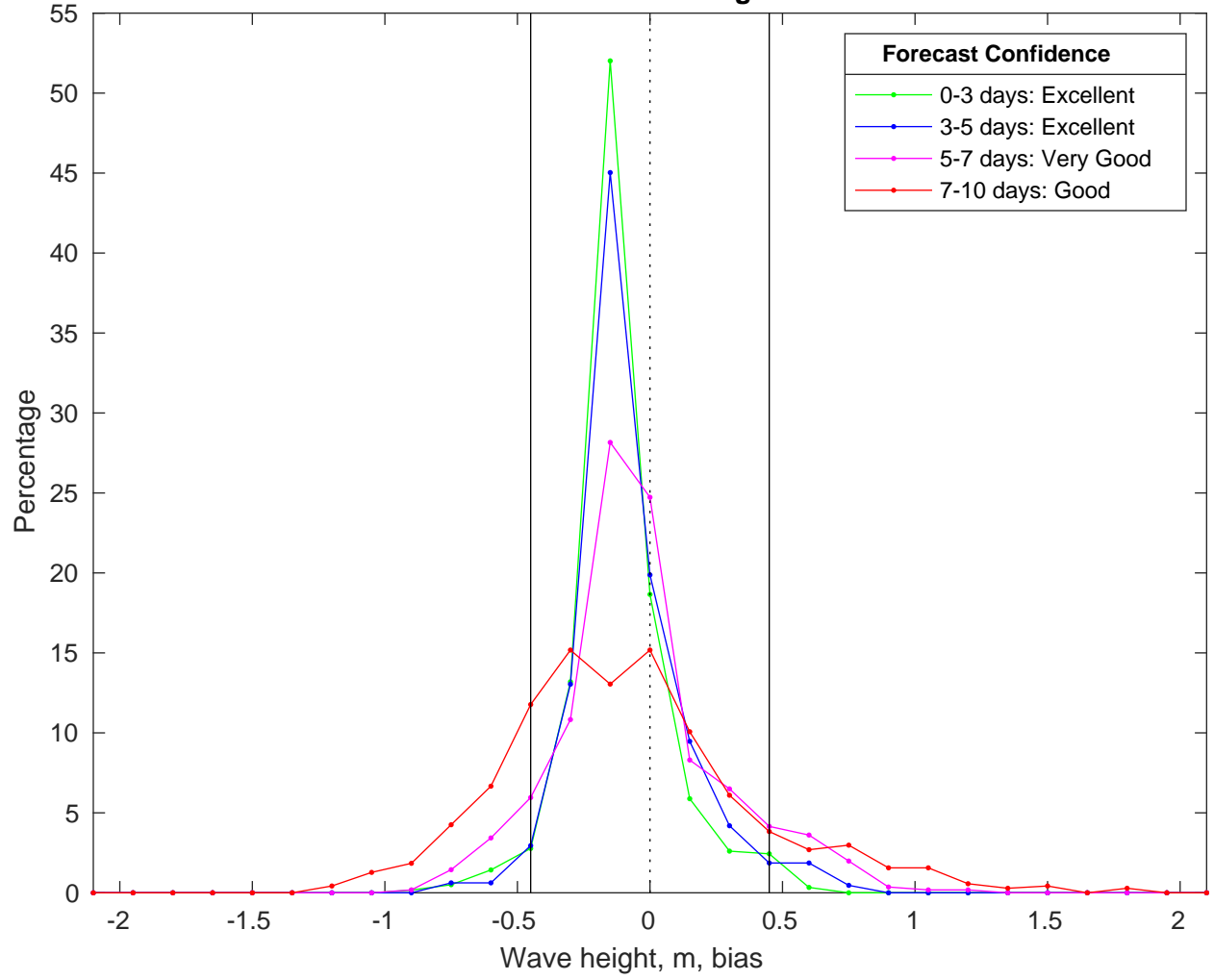
NDBC 42036 vs CMEMS Waves Bias Histogram: 23-Feb-2025
