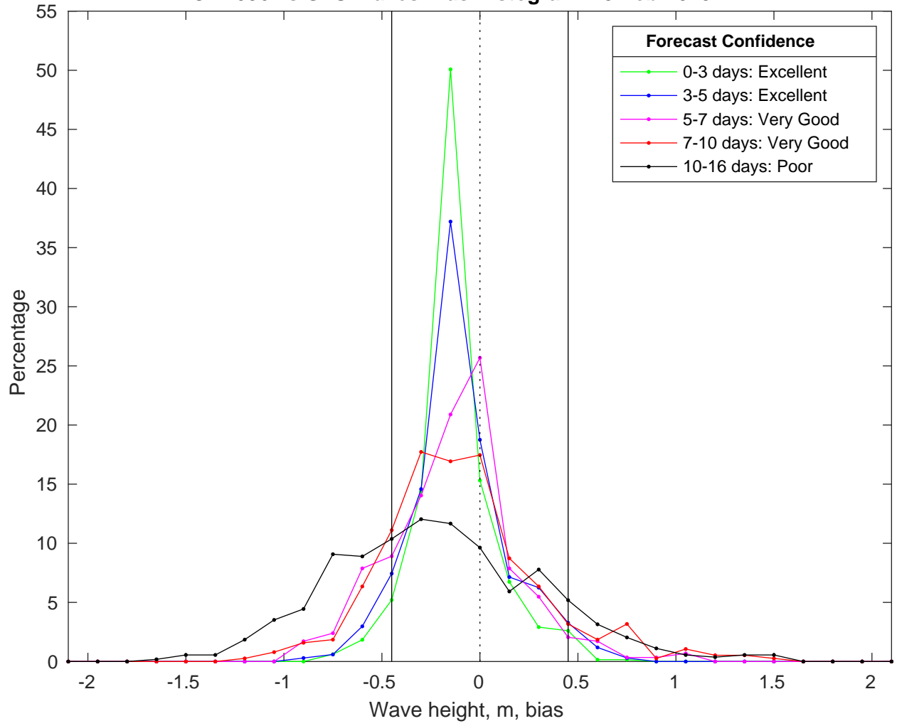
NDBC 42036 vs GFS Waves Bias Histogram: 23-Feb-2025
