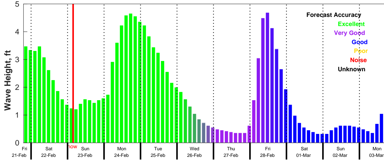
CMEMS Wave Forecast for NDBC 42036 from 21-Feb-2025 19:00:00 to 03-Mar-2025 19:00:00
