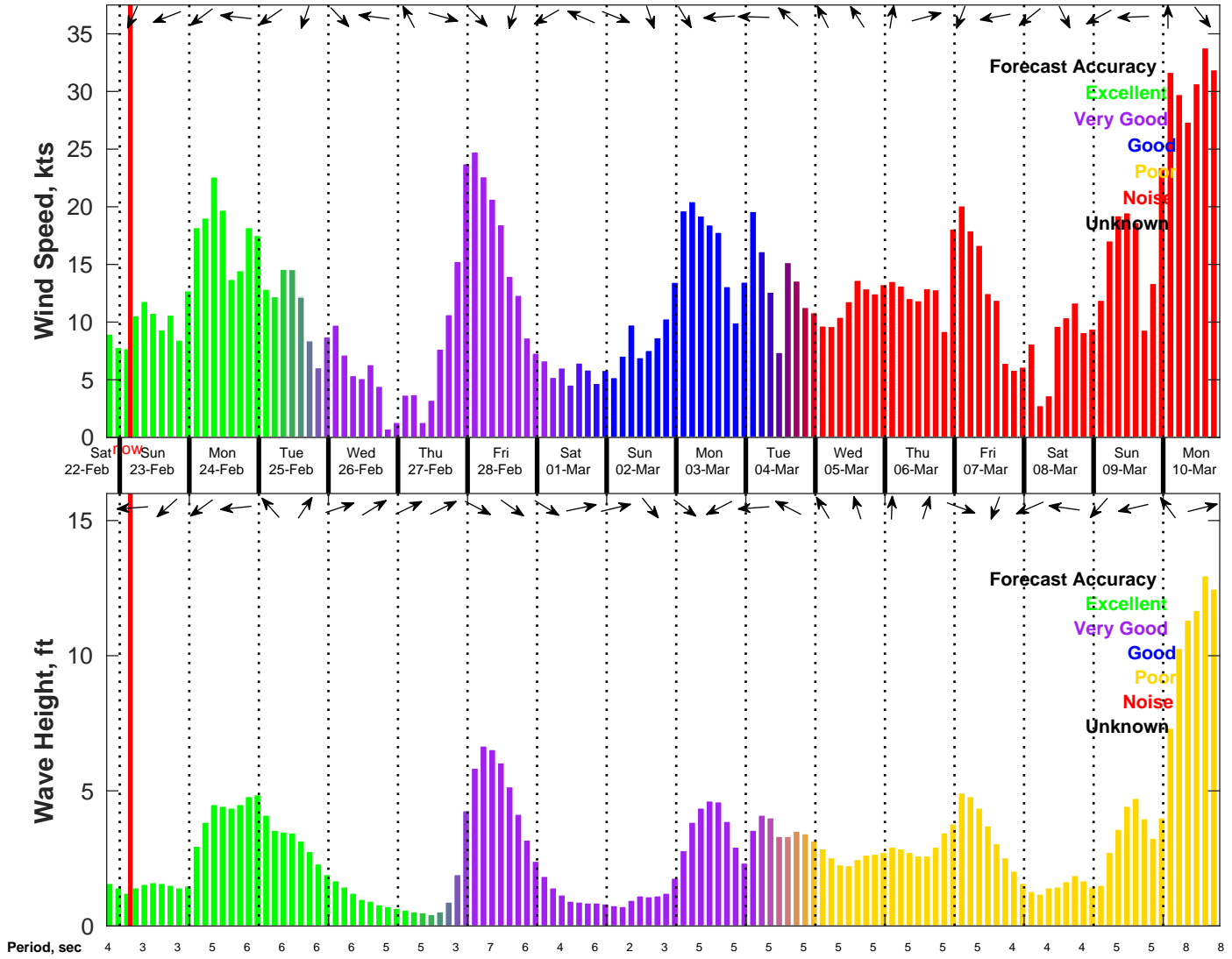
Wind & Wave Forecast for NDBC 42036 from 22-Feb-2025 19:00:00 to 10-Mar-2025 19:00:00
