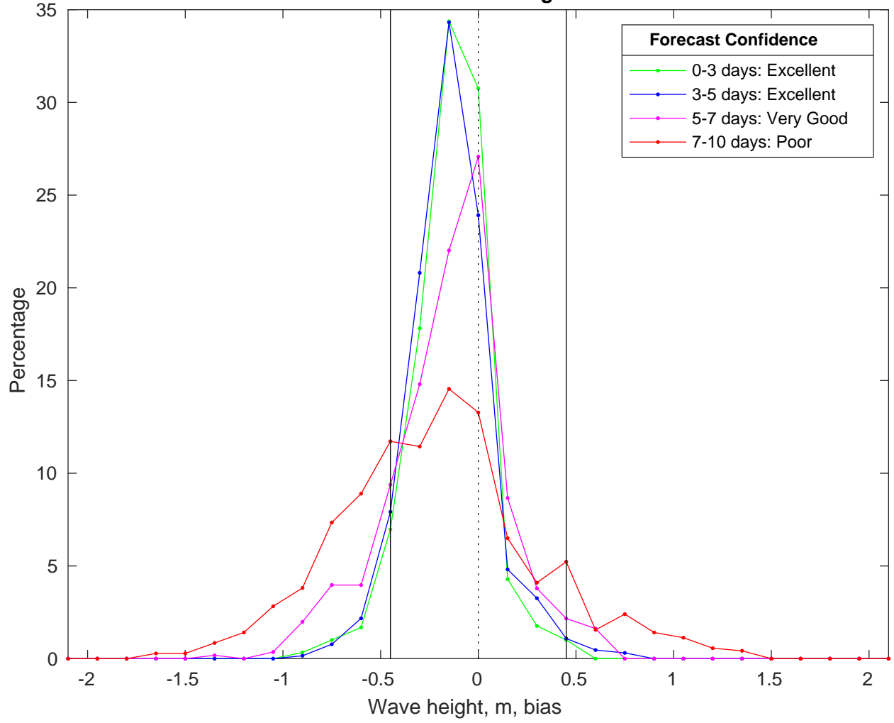
NDBC 42040 vs CMEMS Waves Bias Histogram: 23-Feb-2025
