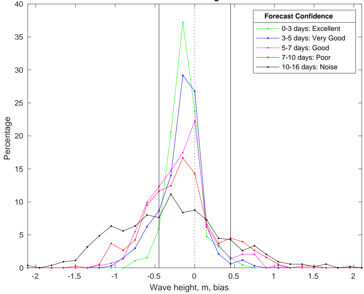
NDBC 42040 vs GFS Waves Bias Histogram: 23-Feb-2025
