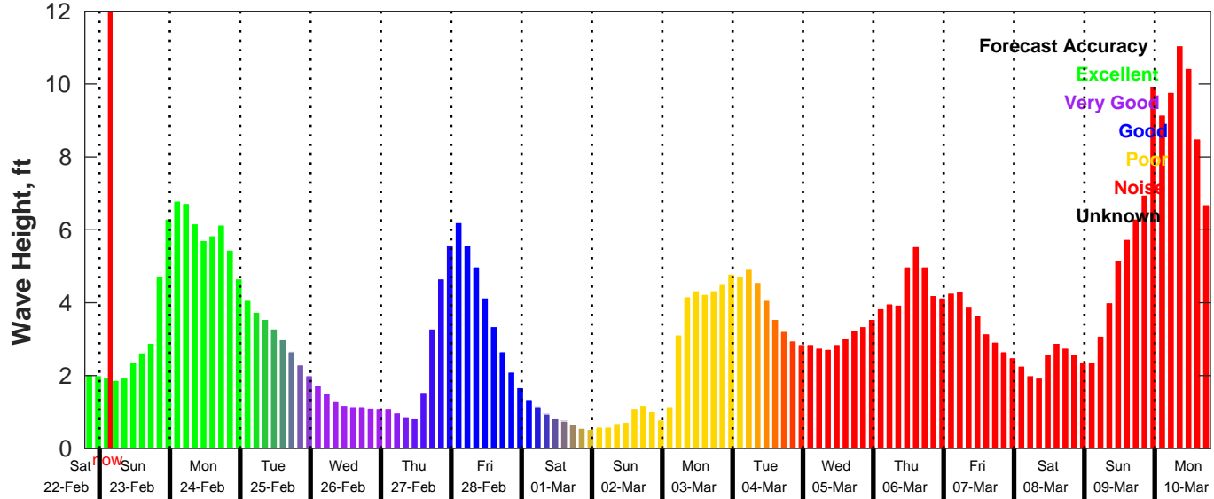
GFS Wave Forecast for NDBC 42040 from 22-Feb-2025 19:00:00 to 10-Mar-2025 19:00:00
