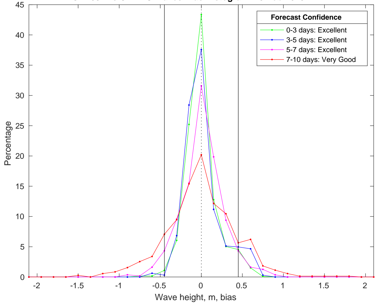
NDBC 42084 vs CMEMS Waves Bias Histogram: 23-Feb-2025
