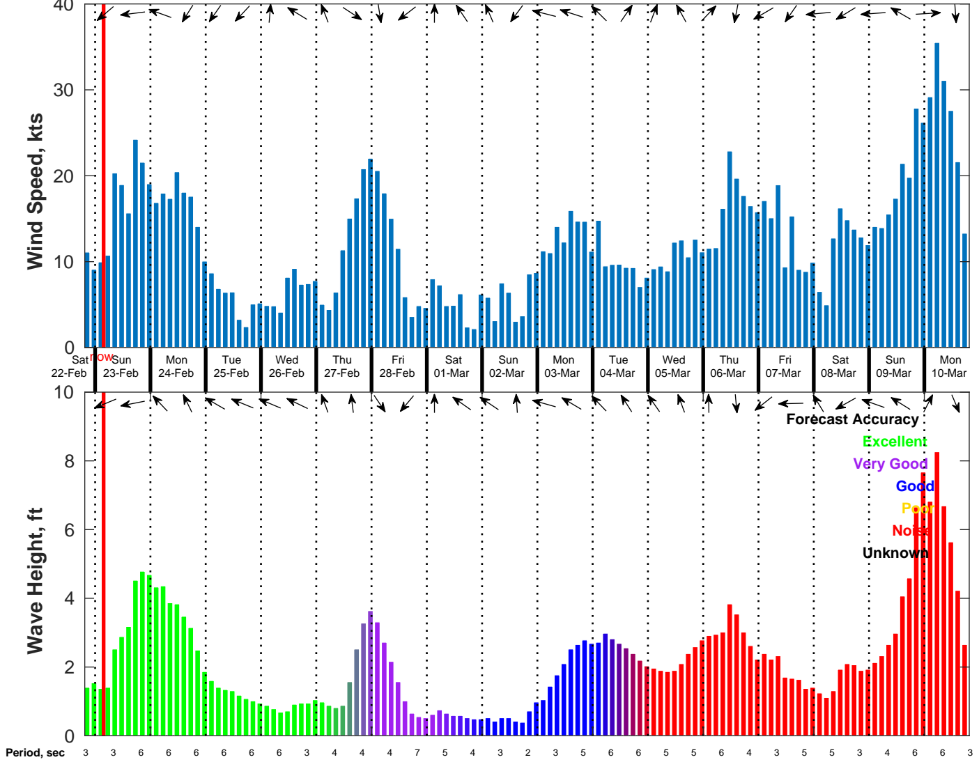
Wind & Wave Forecast for NDBC 42084 from 22-Feb-2025 19:00:00 to 10-Mar-2025 19:00:00
