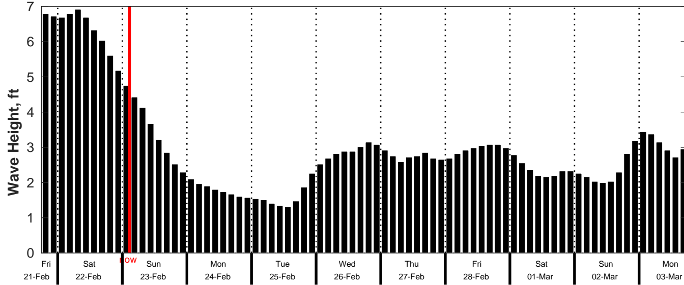
CMEMS Wave Forecast for NDBC 42092 from 21-Feb-2025 18:00:00 to 03-Mar-2025 18:00:00
