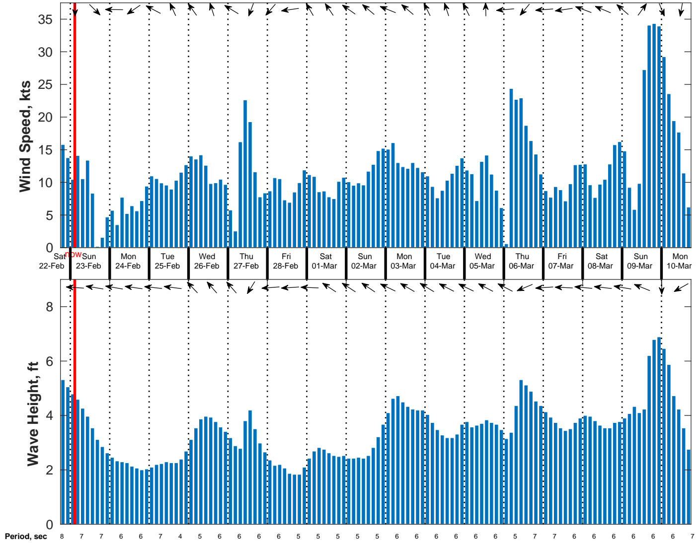
Wind & Wave Forecast for NDBC 42092 from 22-Feb-2025 18:00:00 to 10-Mar-2025 18:00:00
