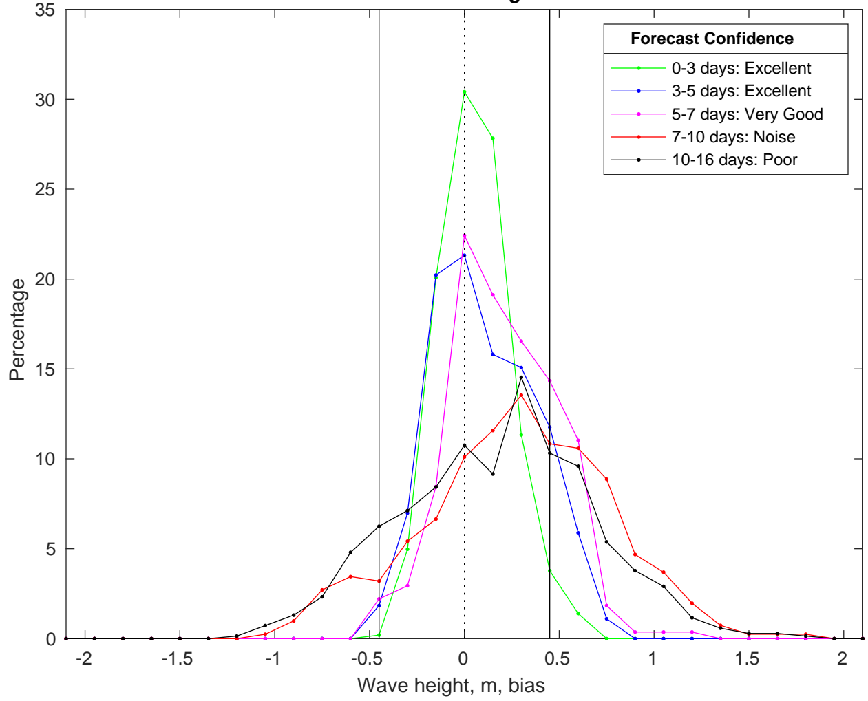
NDBC 44020 vs GFSWaves Bias Histogram: 03-Feb-2025
