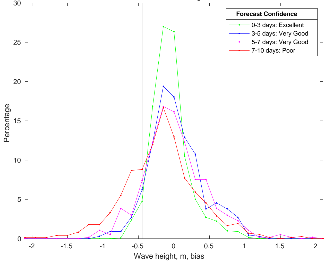
NDBC 46011 vs CMEMS Waves Bias Histogram: 23-Feb-2025
