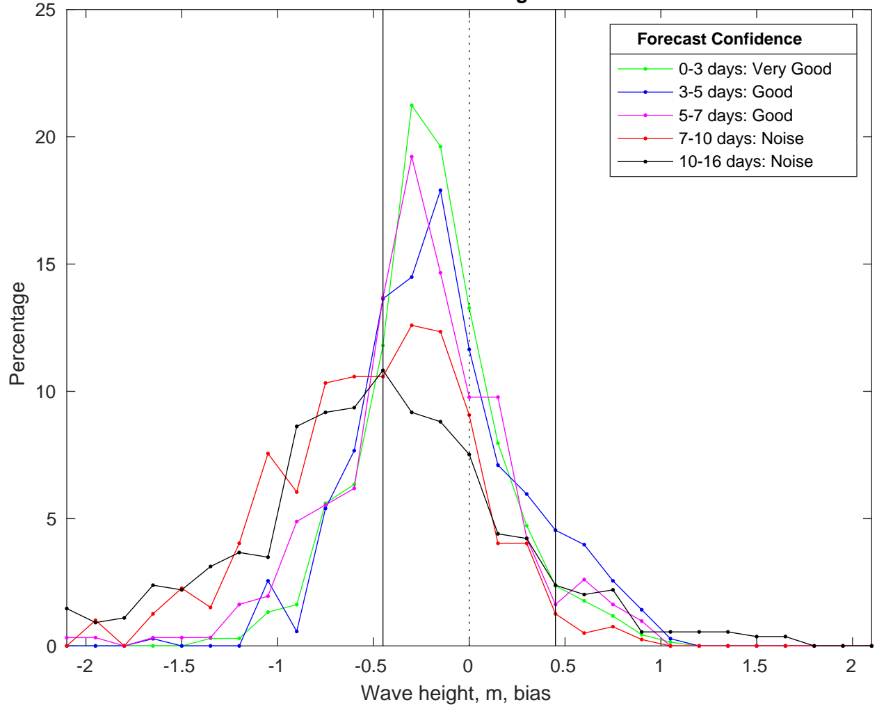
NDBC 46011 vs GFS Waves Bias Histogram: 23-Feb-2025
