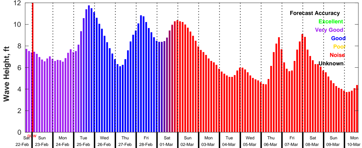
GFS Wave Forecast for NDBC 46011 from 22-Feb-2025 16:00:00 to 10-Mar-2025 16:00:00
