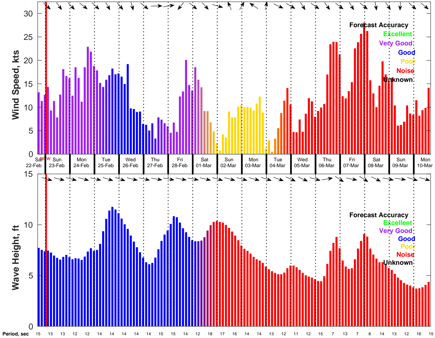
Wind & Wave Forecast for NDBC 46011 from 22-Feb-2025 16:00:00 to 10-Mar-2025 16:00:00
