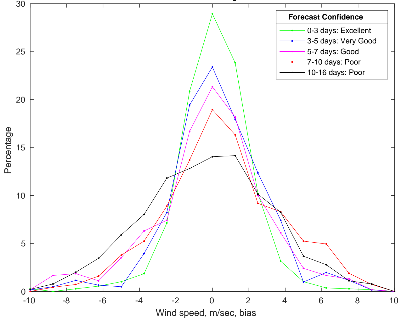
NDBC 46011 vs GFS Winds Bias Histogram: 26-Dec-2024
