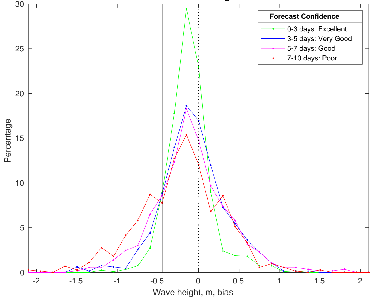
NDBC 46028 vs CMEMS Waves Bias Histogram: 23-Feb-2025
