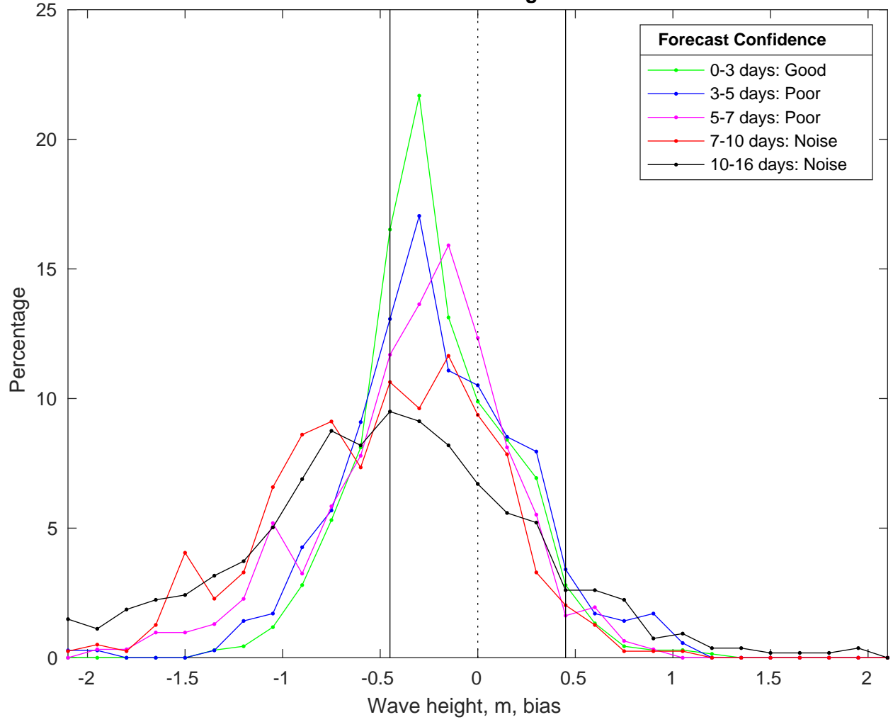
NDBC 46028 vs GFS Waves Bias Histogram: 23-Feb-2025
